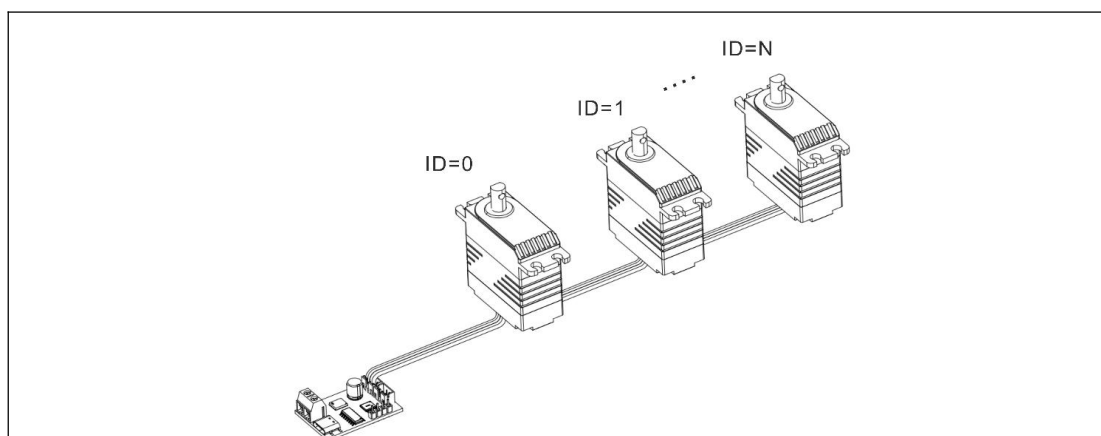
串联
